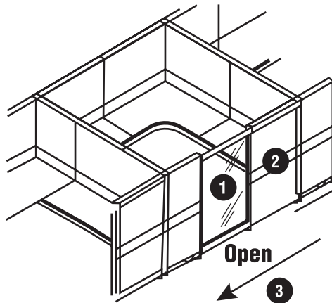
FLAT PRIVACY SCREEN 1. SHOWN IN AN OPEN POSITION 2. MOUNTED ON A 36" PANEL 2. SLIDING LEFT
