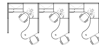
Lay-in Cable Management
